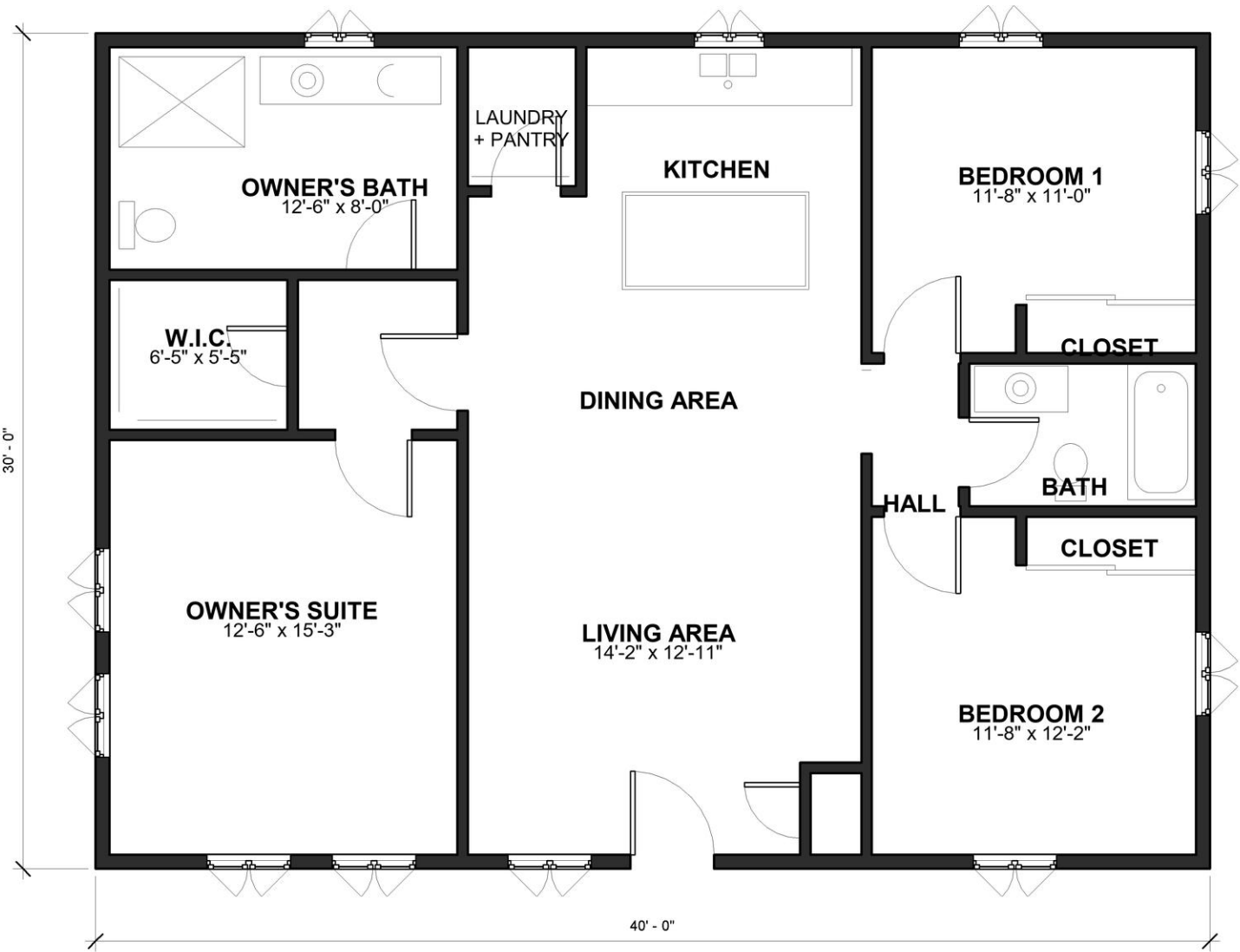
FLOOR PLAN
