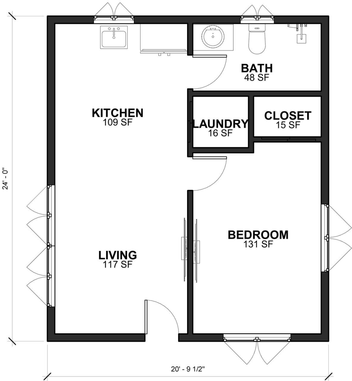
FLOOR PLAN
