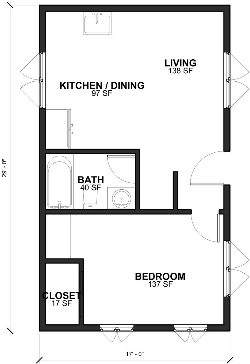
FLOOR PLAN
