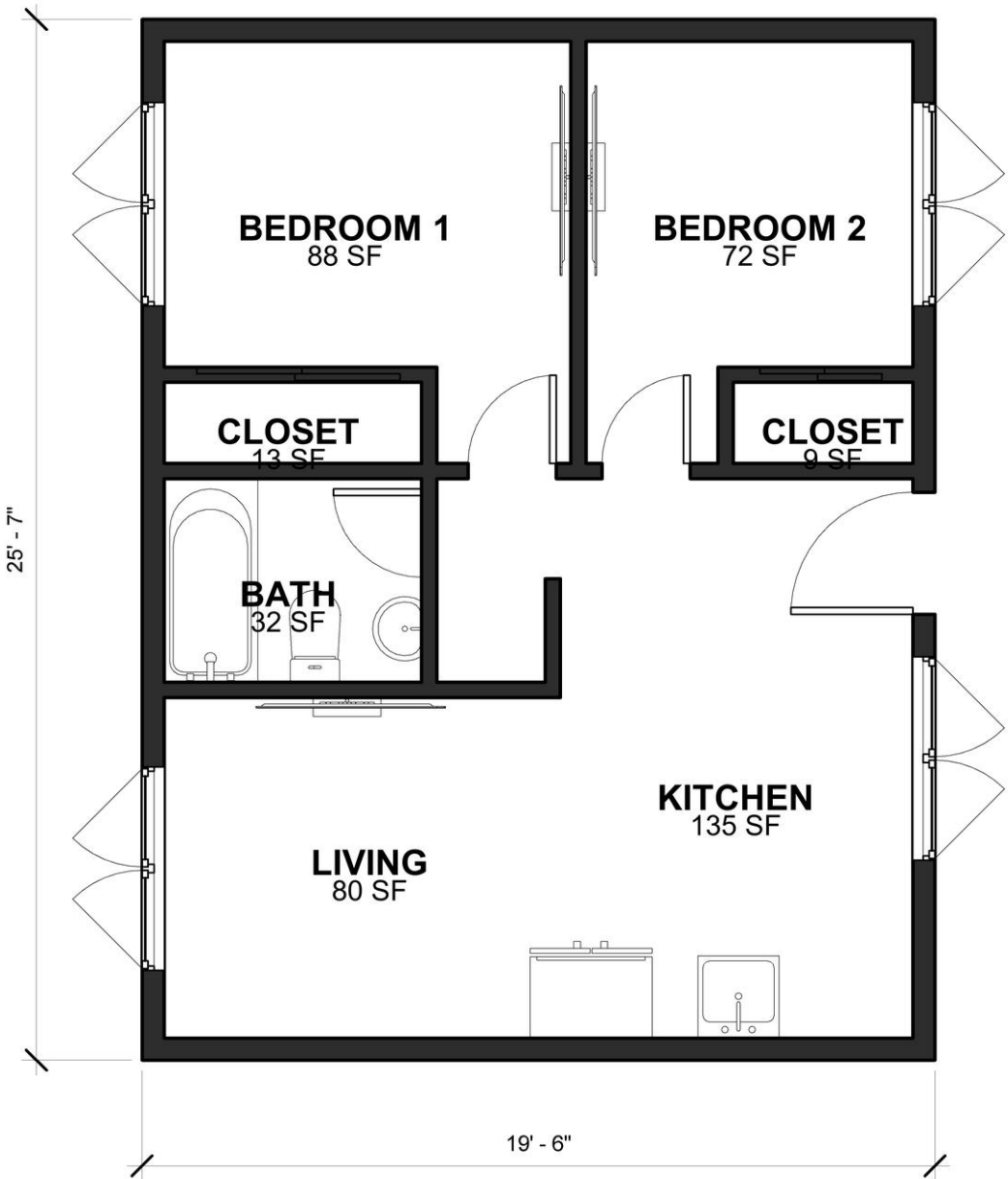
FLOOR PLAN
