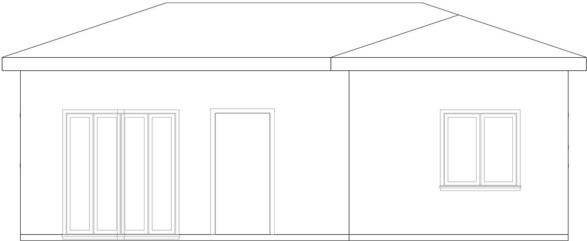
FRONT ELEVATION
