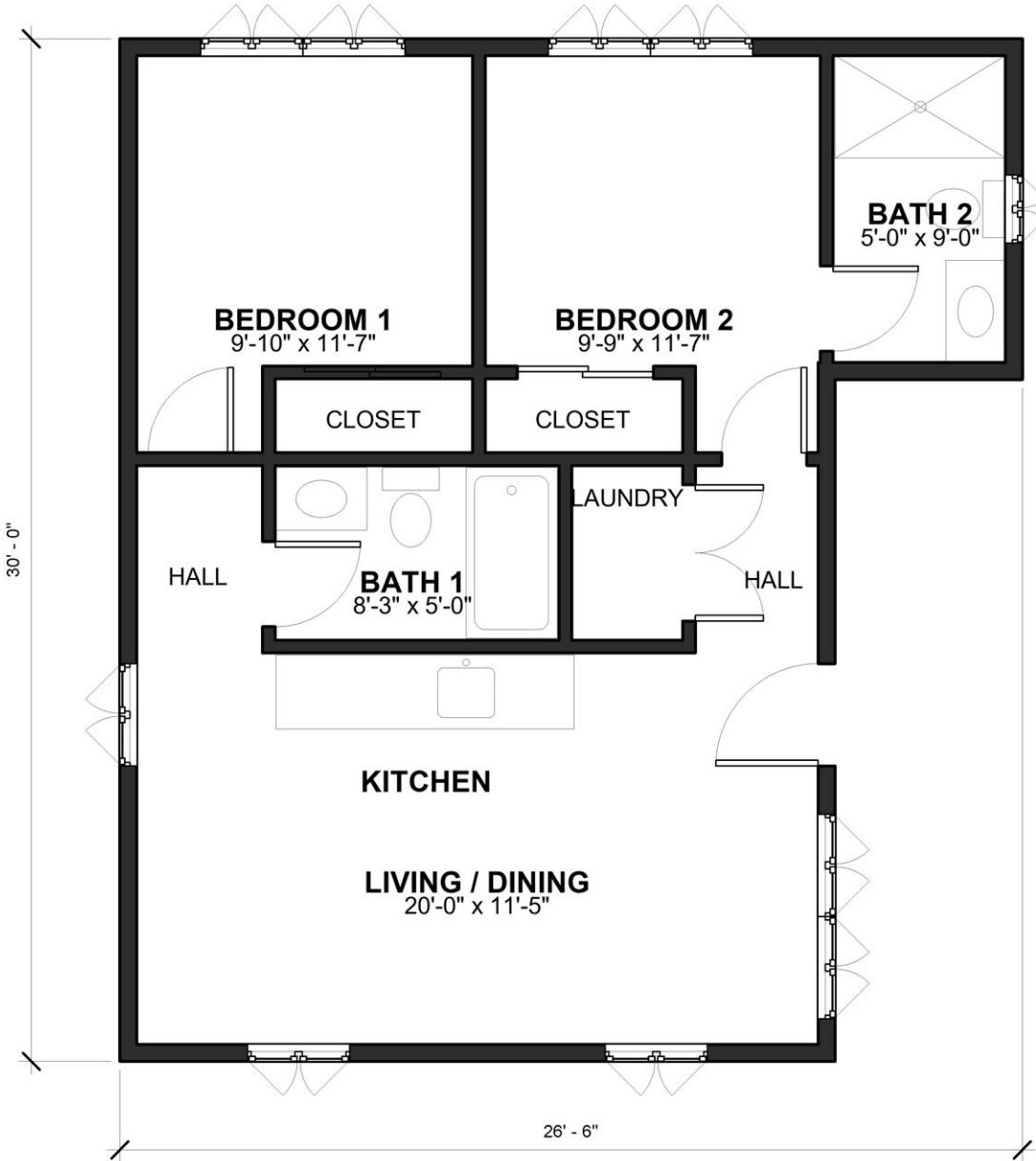
FLOOR PLAN
